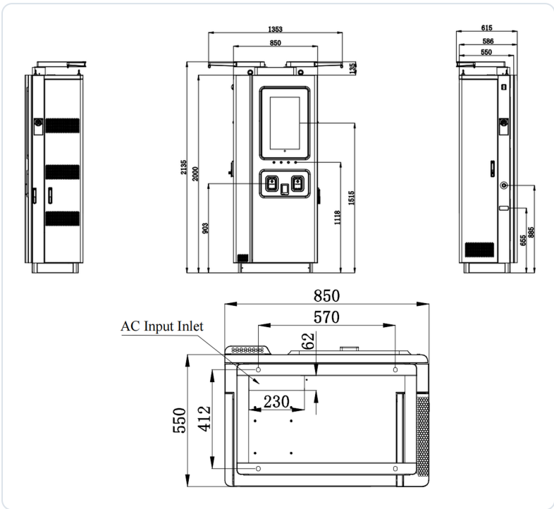
Dimensions in mm. Drawing applies to models PVP120 to PVP240 (identical cabinet). Bottom right: base plate with mounting holes and AC inlet.
